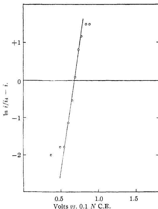
Fig. 5.— \log i/i_a - i vs. cathode potential of 1 \times 10^{-3} benzo(c)cinnoline at an apparent pH of 5.2.
