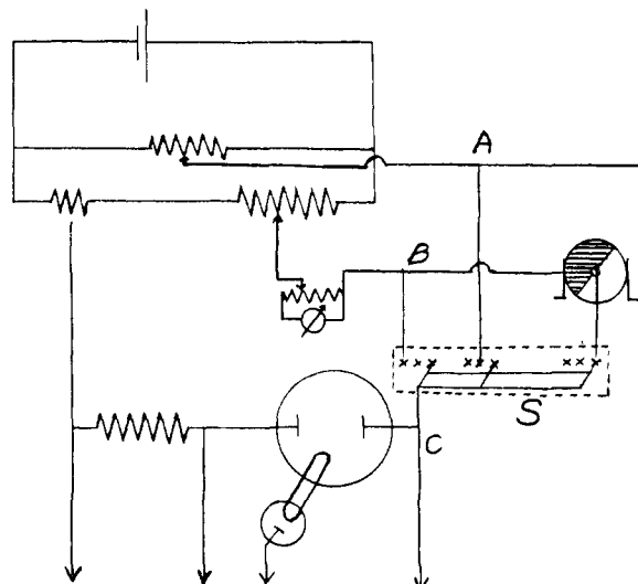
Fig. 10.—Schematic diagram of Lingane and Koltzoff manual polarograph adapted to Kalousek technique (see reference 8).
