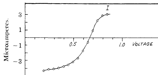
Fig. 6.—Kalousek curve at 1.5 cycles per second obtained for 1 \times 10^{-3} M benzo(c)cinnoline at an apparent pH of 5.2.
