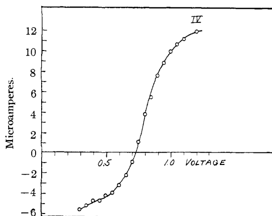
Fig. 9.—Kalousek curve at 30 cycles per second for 1 \times 10^{-3} M 2,2'-dinitrosobiphenyl at an apparent pH of 5.2.
